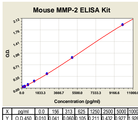
Figure 1: MMP-2 Standard Curve. Using the mouse MMP-2 ELISA Kit, O.D. data was graphed against MMP-2 protein concentration. The TMB reaction was incubated at 37° C for 30 min.
